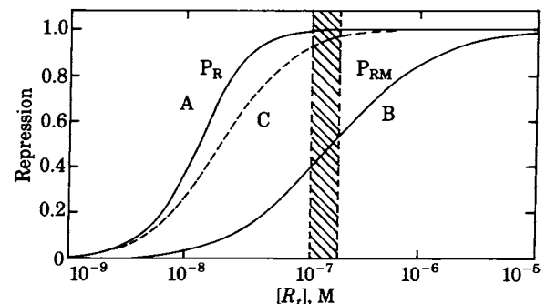
Fig. 2. Predicted repression curves at P_R and P_{RM} . Curve A represents f_{PR} , the probability that an operator template will have O_{R1} , O_{R2} , or both occupied (each of these three configurations shuts off transcription from P_R ) as a function of R_t in units of monomer. This curve includes all effects of cooperative interaction between repressor dimers bound to adjacent operator sites and also of repressor dimer dissociation into inactive monomers. Curve B represents f_{PRM} , the probability that O_{R3} is occupied (required for shutoff of transcription at P_{RM} ), including all effects. Curve C, repression curve for P_R devoid of cooperative interactions. \square , Approximate concentration of repressor in a lysogenic cell.
