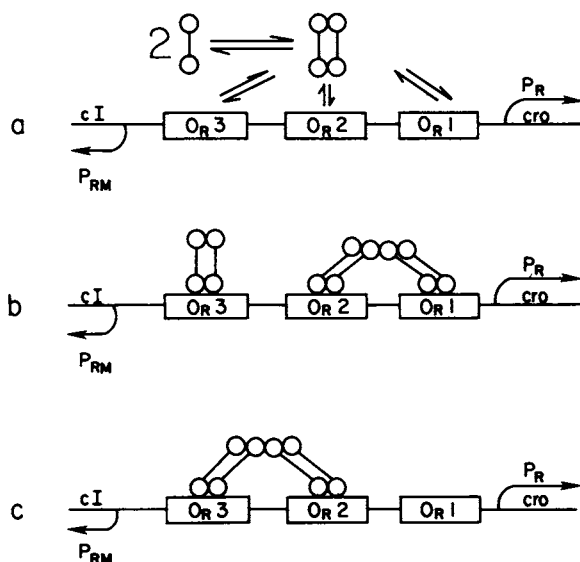
FIG. 1. Interactions of repressor molecules (○—○) at the right operator, O R , of the \lambda phage genome. The DNA binding sites for repressor (designated O R 1, O R 2, and O R 3) are each composed of 17 base pairs and are separated by spacers of 6 and 7 base pairs. Binding of repressor molecules controls transcription by RNA polymerase from the two divergent promoters, P R and P RM . Transcription of the cro gene from P R and consequent synthesis of cro protein leads to lytic growth of the phage genome and cell lysis. Transcription of the cl gene from the promoter P RM and consequent synthesis of repressor is required to maintain the lysogenic state by preventing cro synthesis. (a) Active repressor dimers in equilibrium with inactive monomers. The dimers bind reversibly to each of the three operator sites (arrows). Binding can result in any of the seven combinations shown in Table 1. (b and c) Types of cooperative interaction believed to occur between adjacent bound repressors (configurations 7 and 8 of Table 1).
